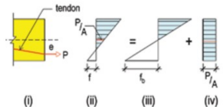
Figure 1b. Distribution of stress from post-tensioning on a section. P/A is the average precompression; f_b is the extreme fiber stress from post-tensioning moment, M_{pt} . P is the post-tensioning force and e is the eccentricity of the force with respect to the section's centroid.
