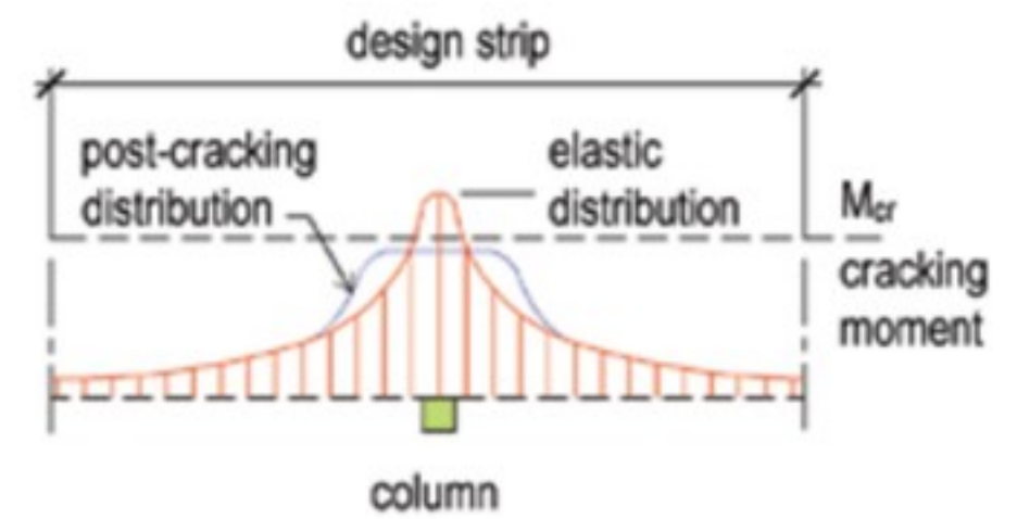
Figure 3. Plan – Tributary (design strip) of a column support in two-way slab construction. Distribution of moment at the face of column before and after cracking. Loss of capacity due to the cracking spreads the cracking and mobilizes the slab’s strength beyond the column (PTS761).
