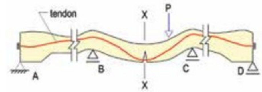
Figure 1a. Partial elevation; continuous member reinforced with post-tensioning forces leading to cracking at section X-X depend on the overall geometry of the entire structure, features of its post-tensioning tendons and the applied load (PTS798).
